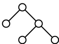
Active Directory
